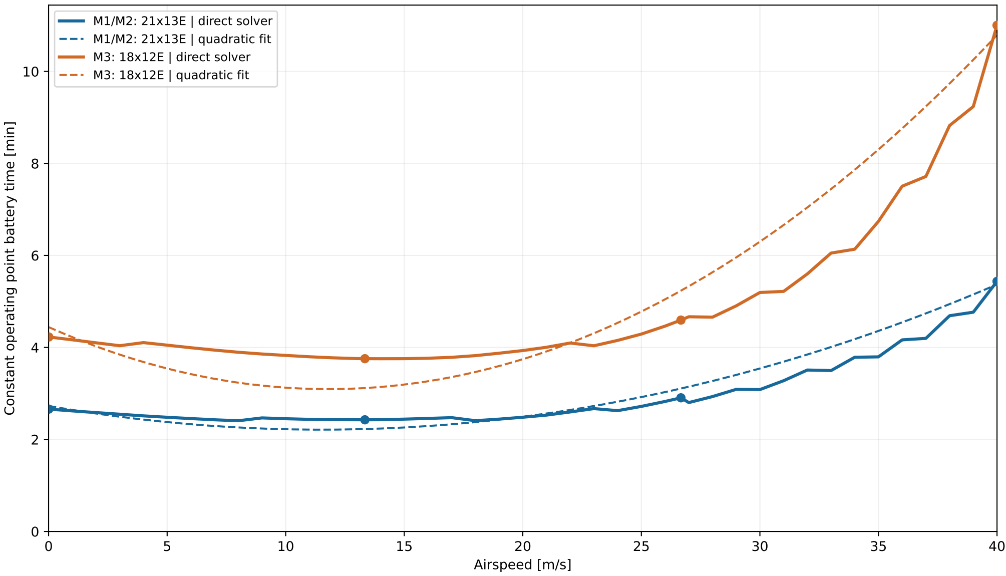
Battery time at maximum available thrust 8S, 3.3714 Ah, 85% usable capacity, throttle cap 1.0
