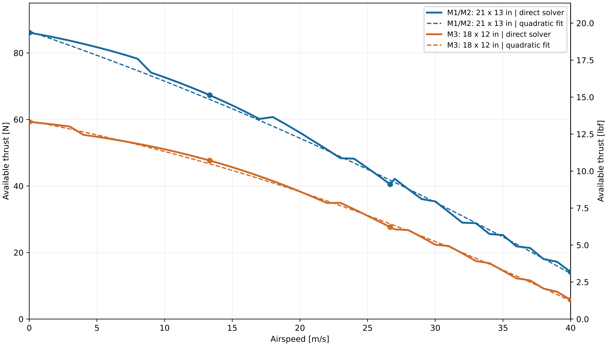
Optimized plane | thrust versus airspeed 8S, 3.3714 Ah, 243.606 Kv, throttle cap 1.0
