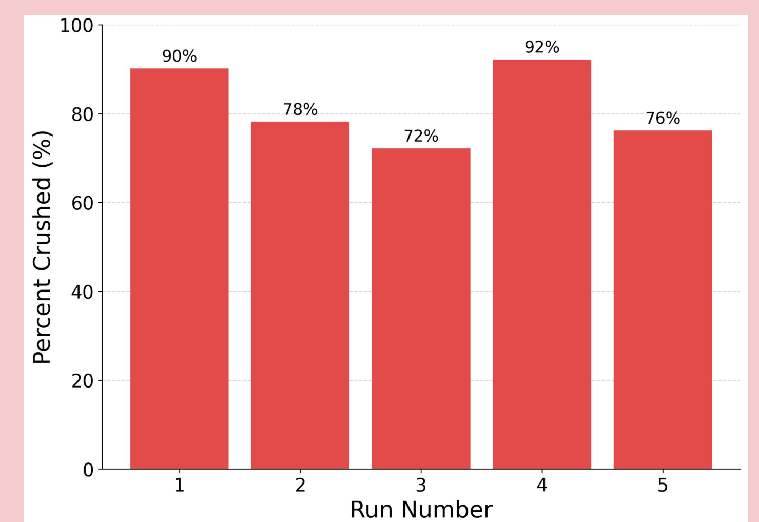
Fig. 5: Plot of Trial 1: 50 SLF Eggs for 90 Seconds. Crushing efficiency ranged from 72% to 92% over five runs, with generally high efficiency and some variability between trials.
