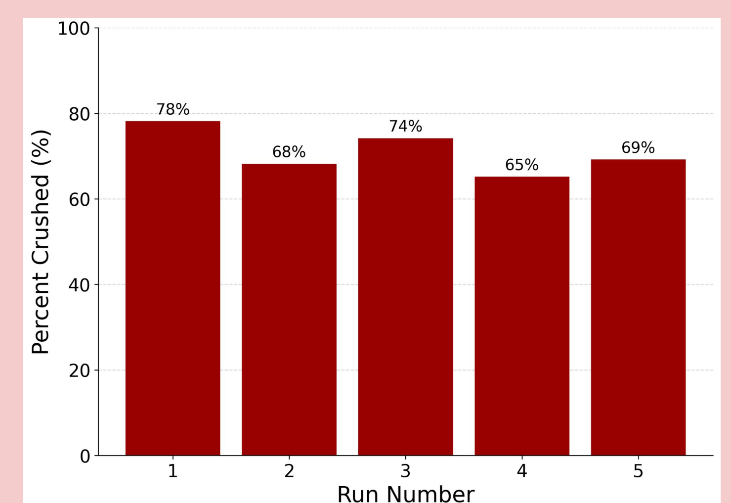
Fig. 7: Plot of Trial 3: 100 SLF Eggs for 3 Minutes. Crushing efficiency ranged from 65% to 78%, showing little to no improvement compared to the 90-second trials.
