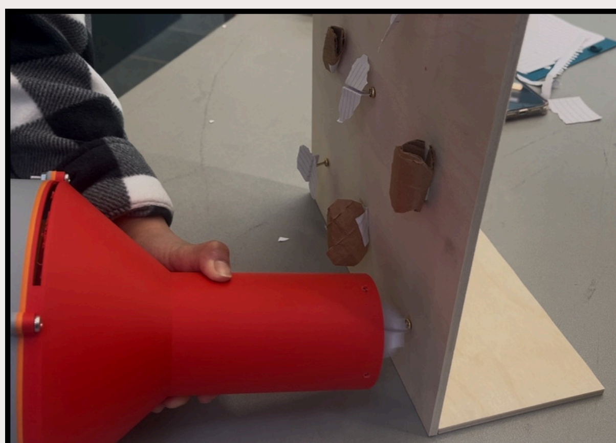
Fig. 6: Testing of the final prototype with the impeller and without the cone.
