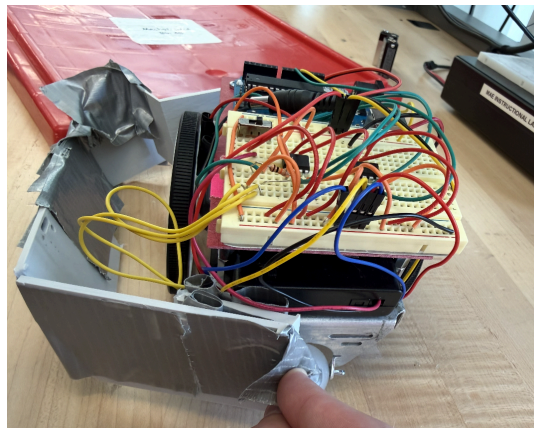
Figure 2: Final Design for our Robot Back View
