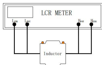
Ls & RDC test schematic diagram
