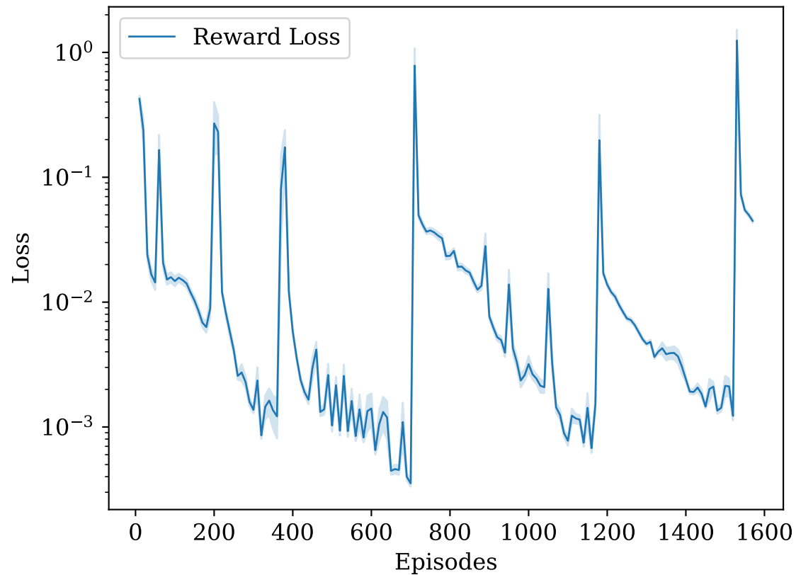
Breakout Reward Loss
