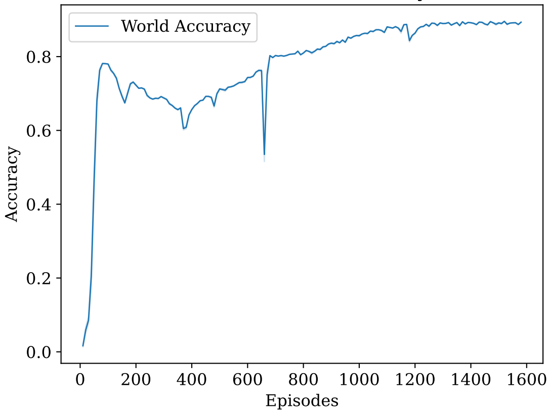
Breakout World Accuracy
