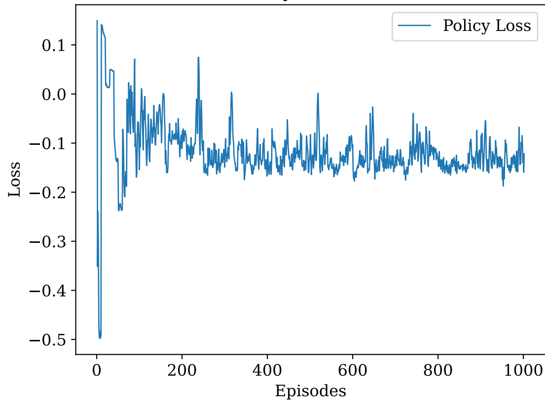
Breakout Policy Loss (transformer)
