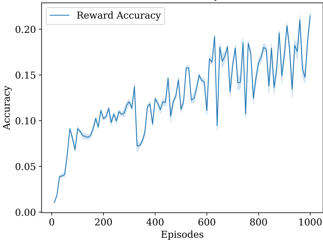
Breakout Reward Accuracy (transformer)
