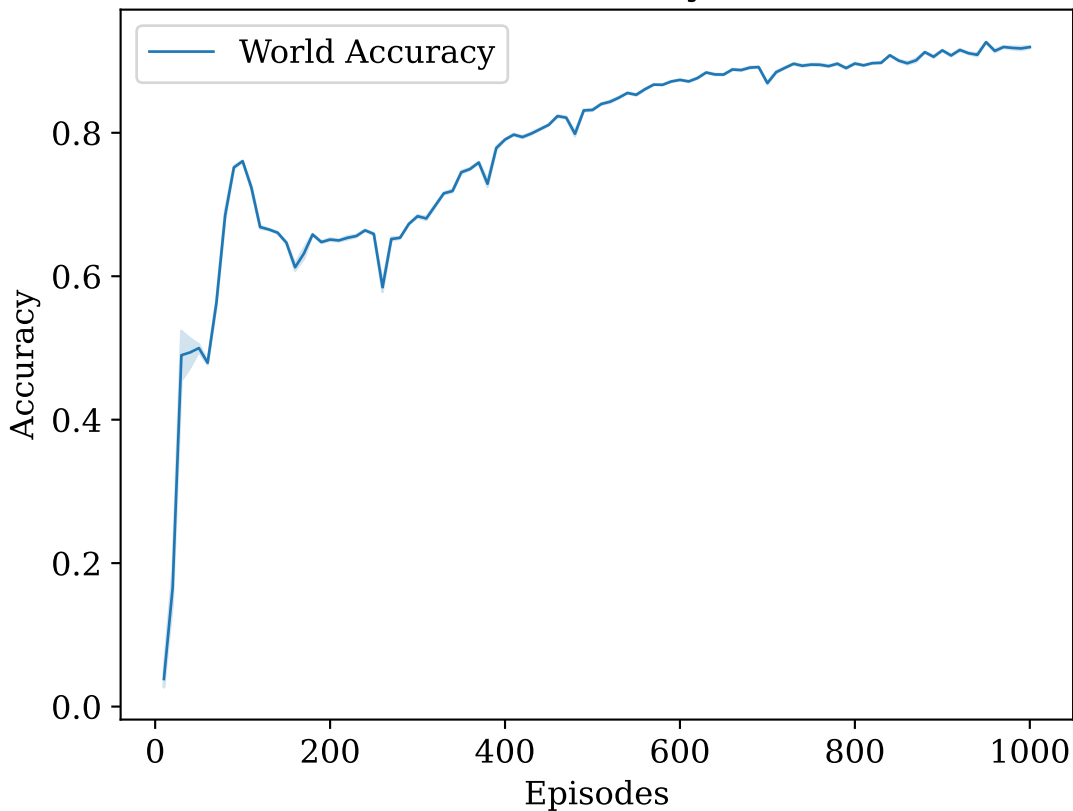
Breakout World Accuracy (transformer)
