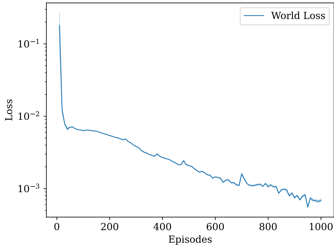
Breakout World Loss (transformer)
