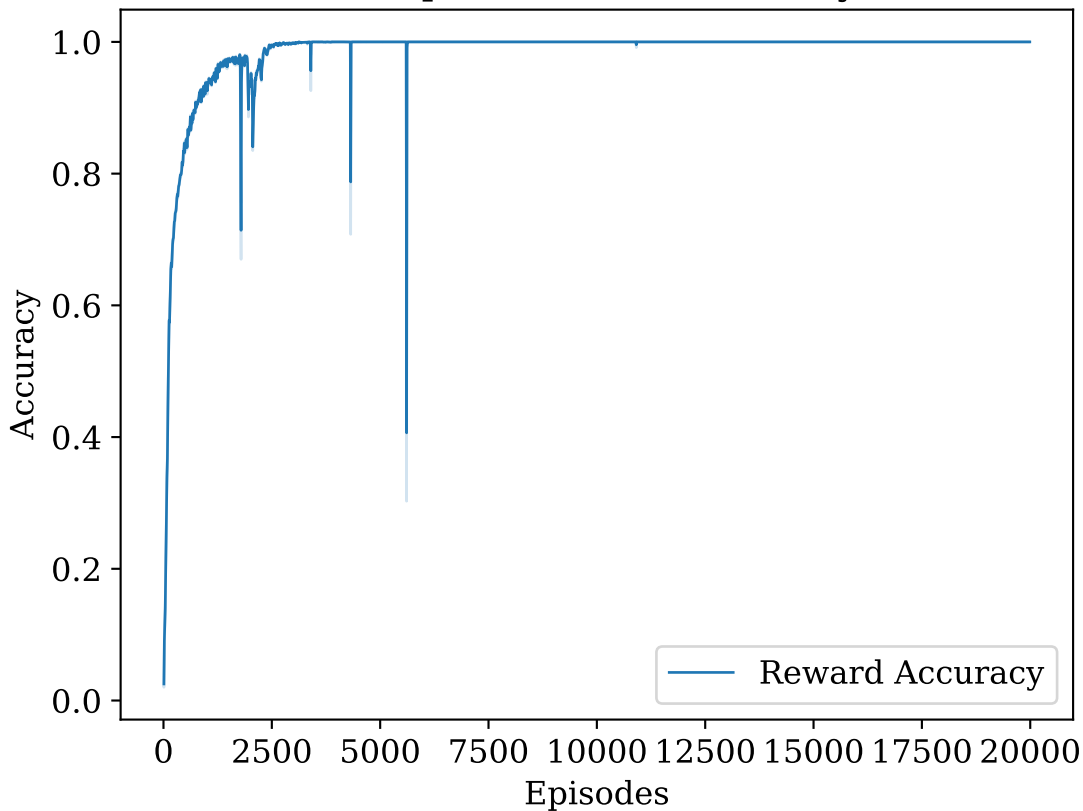
Cartpole Reward Accuracy
