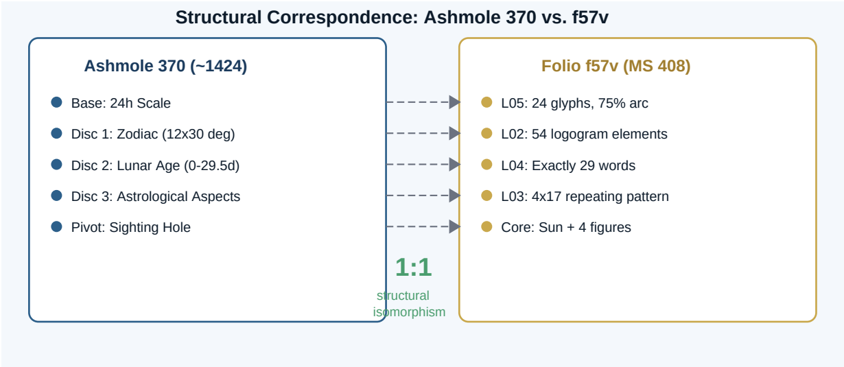
Figure 3. Structural correspondence with Ashmole 370 (~1424). The 29-word ring L04 matches the synodic lunar month.
