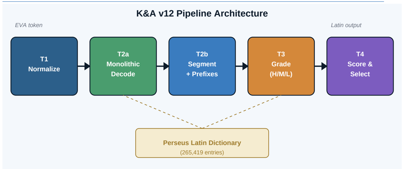
Figure 1. K&A v12 pipeline architecture.
