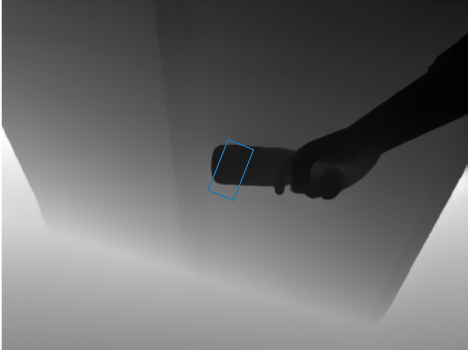
Depth + Grasp
