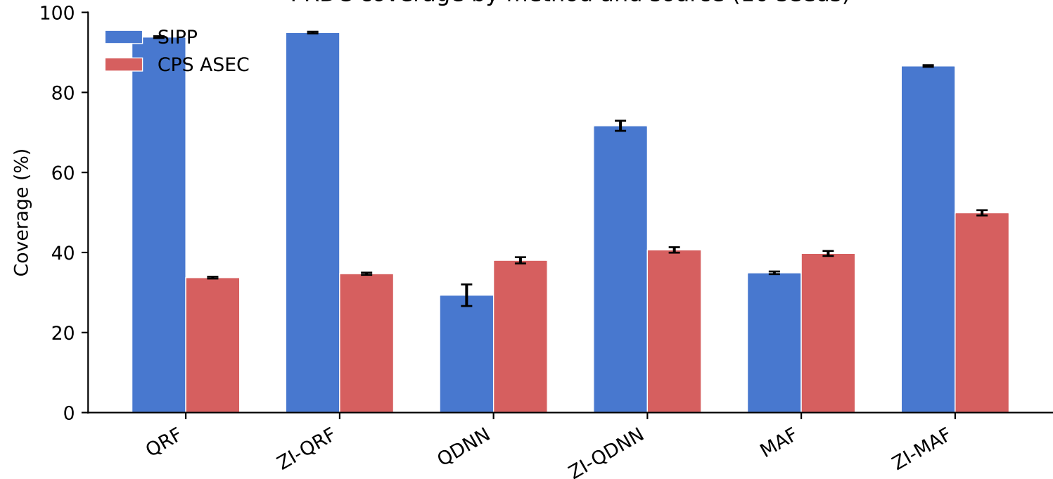
PRDC coverage by method and source (10 seeds)
