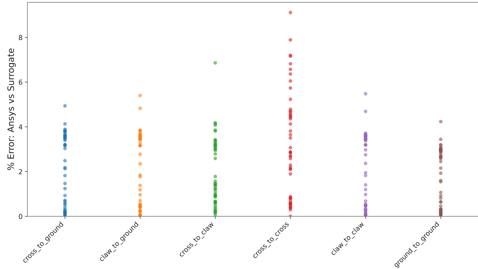
Per-Capacitance Error: Ansys vs Surrogate Prediction (all sigmas)
