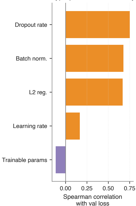
Hyperparameter sensitivity
