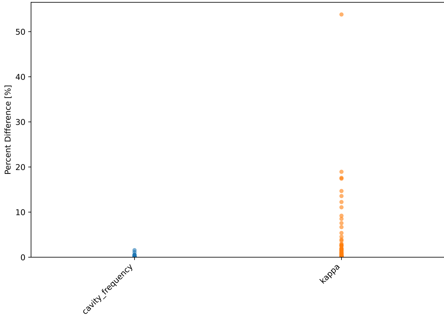
Percent Difference: eigenmode
