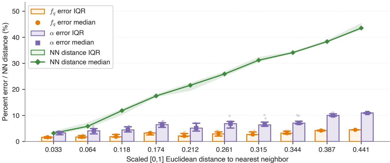
Anslys vs surrogate Hamiltonian error
