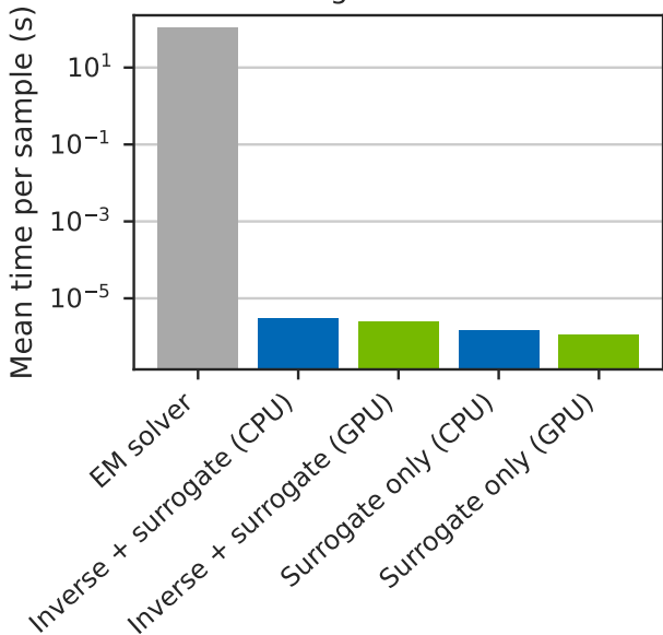
Conventional EM solver vs surrogate inference
