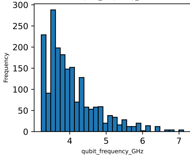
X: qubit_frequency_GHz
