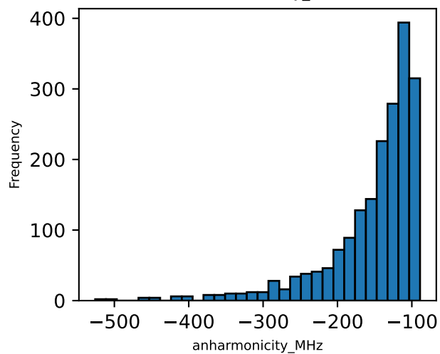
X: anharmonicity_MHz
