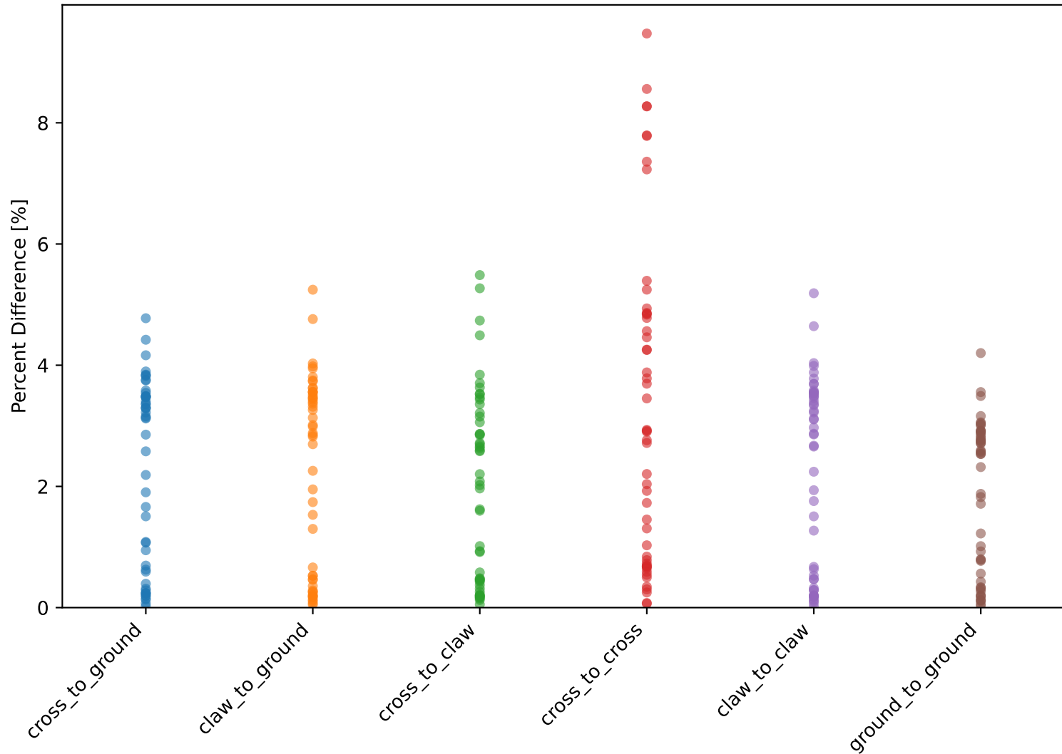
Ansys Simulated Capacitance vs Target Capacitance
