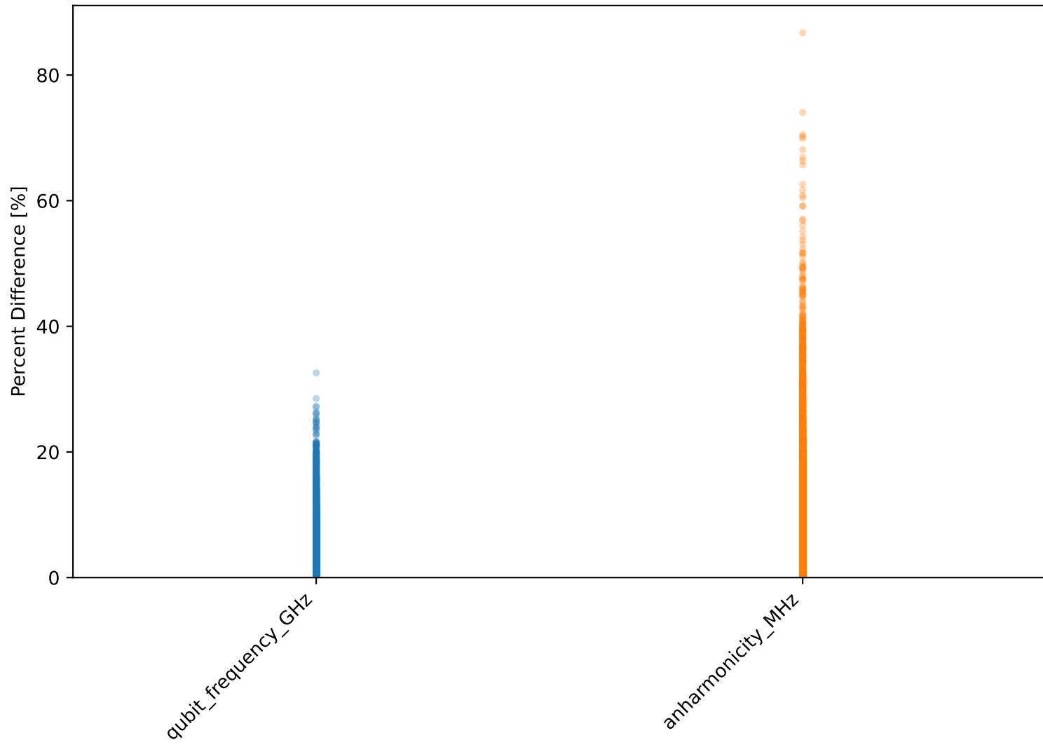
Surrogate % Error — Sigma = 10% of param range
