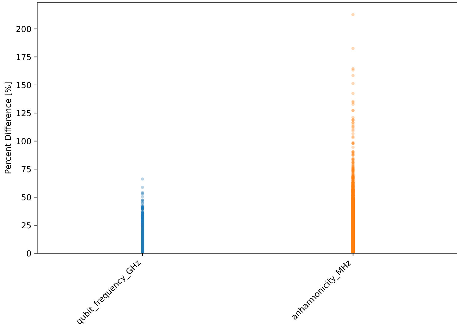
Surrogate % Error — Sigma = 20% of param range
