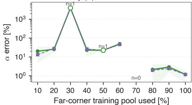
Anharmonicity ( \alpha )
