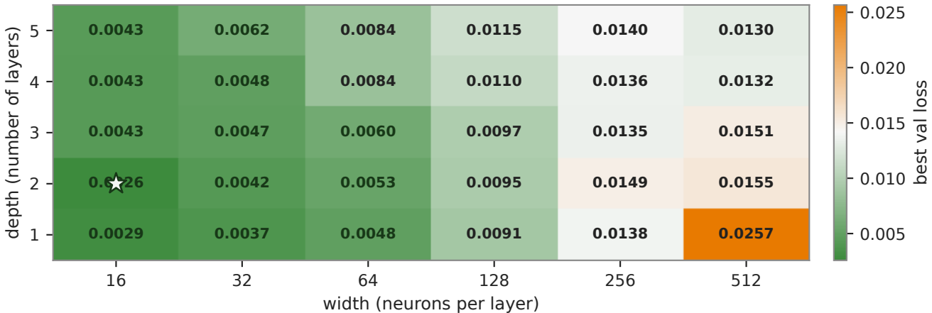
Validation loss
