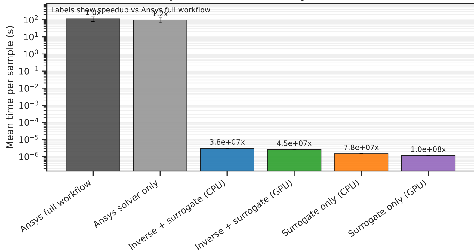
Ansys simulation time vs surrogate inference
