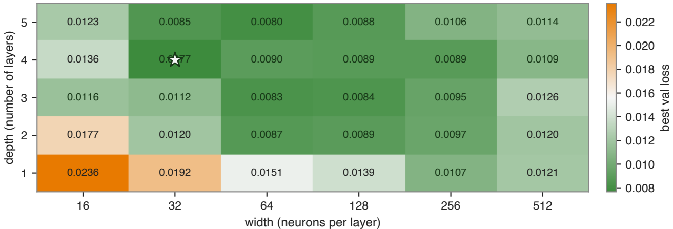
Validation loss
