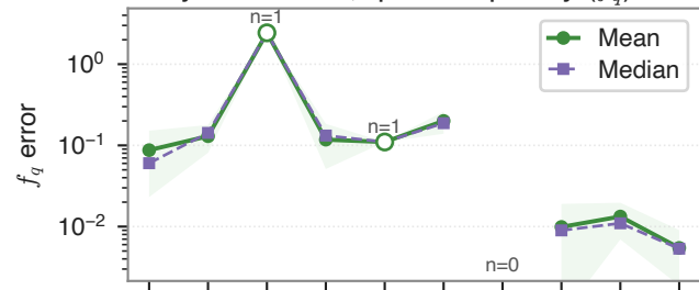
Ansys validation, qubit frequency ( f_q )
