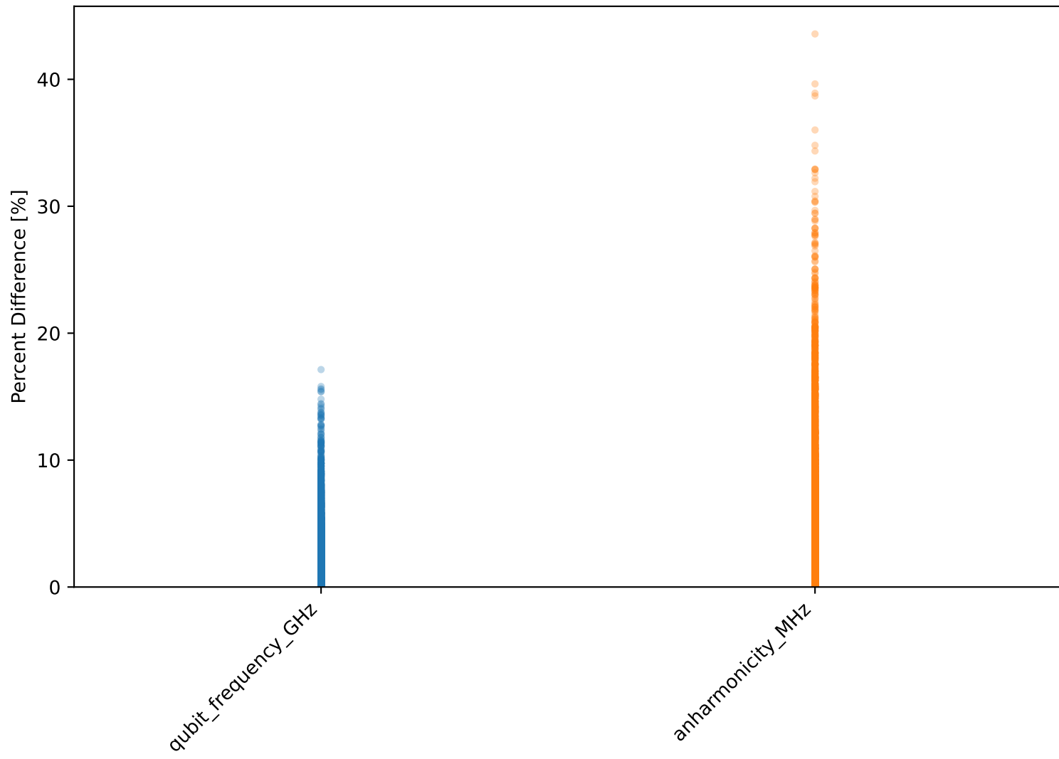
Surrogate % Error — Sigma = 5% of param range
