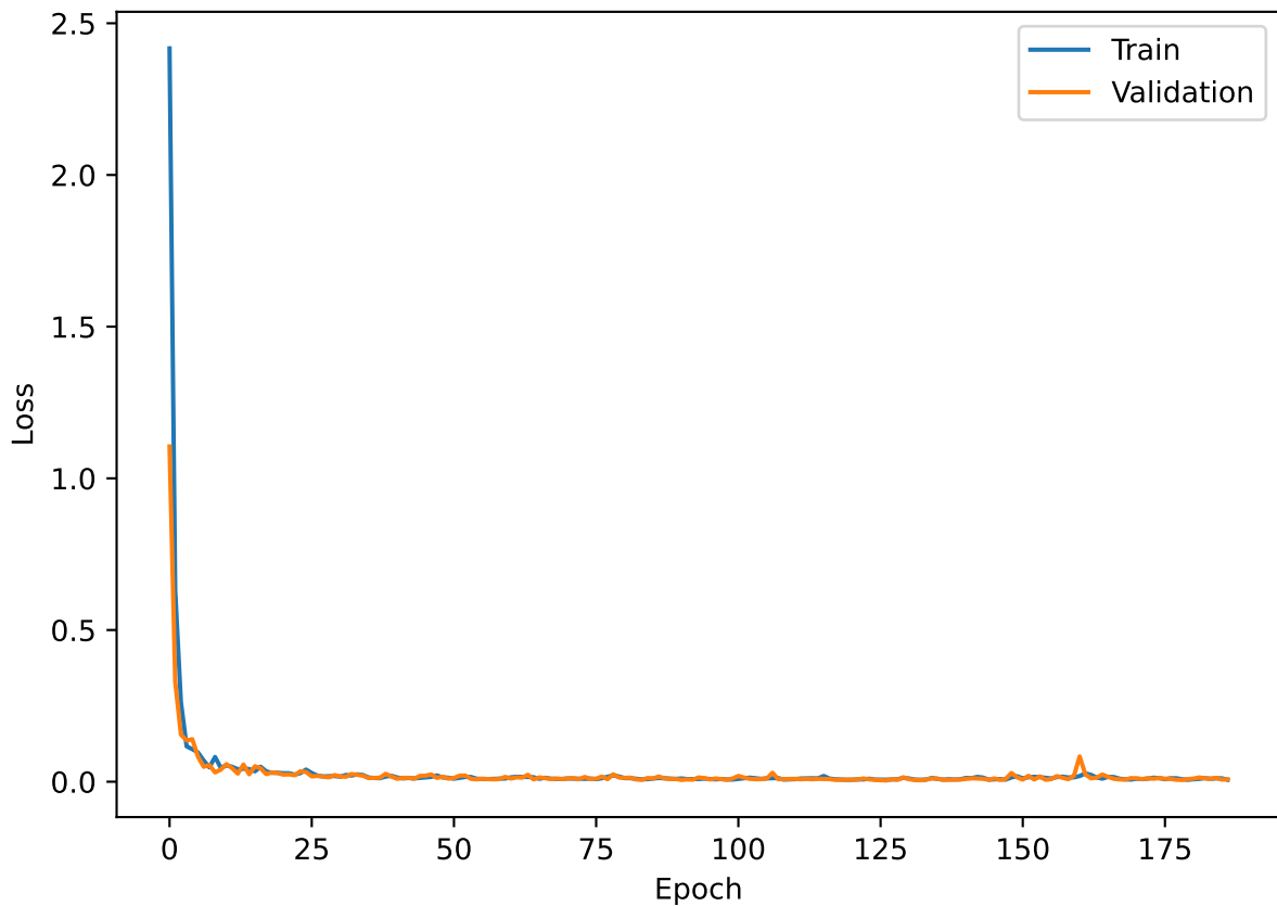
Model 2 loss
