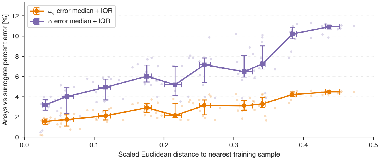
Ansys vs surrogate Hamiltonian error
