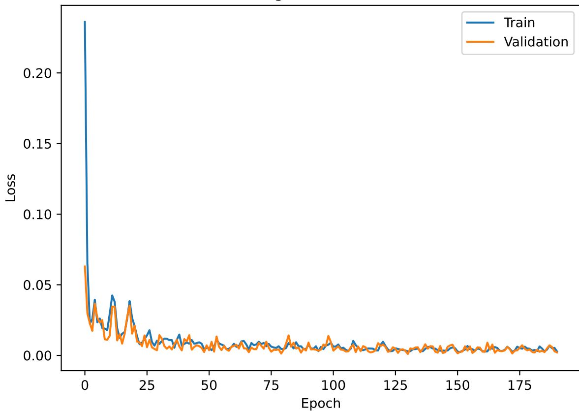
Surrogate-defined loss
