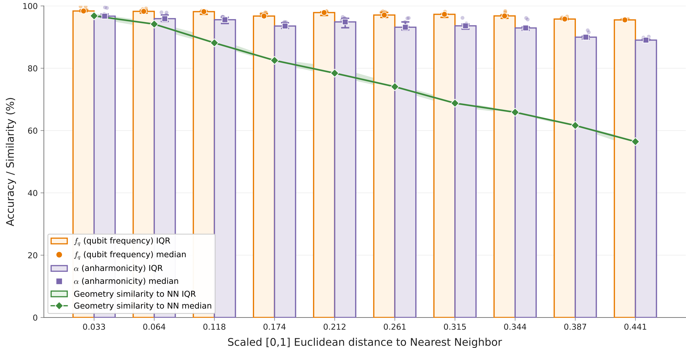
Ansyz vs Surrogate Prediction accuracy of Hamiltonian parameters
