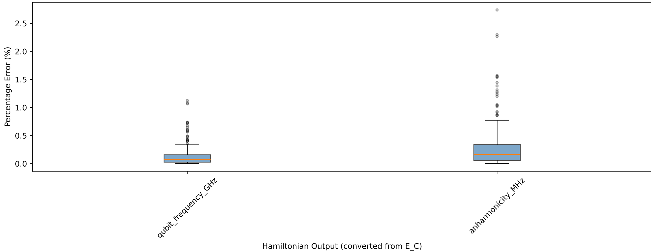
Model 2: Percentage Error Distribution per Output (E_C converted to f_q , \alpha )
