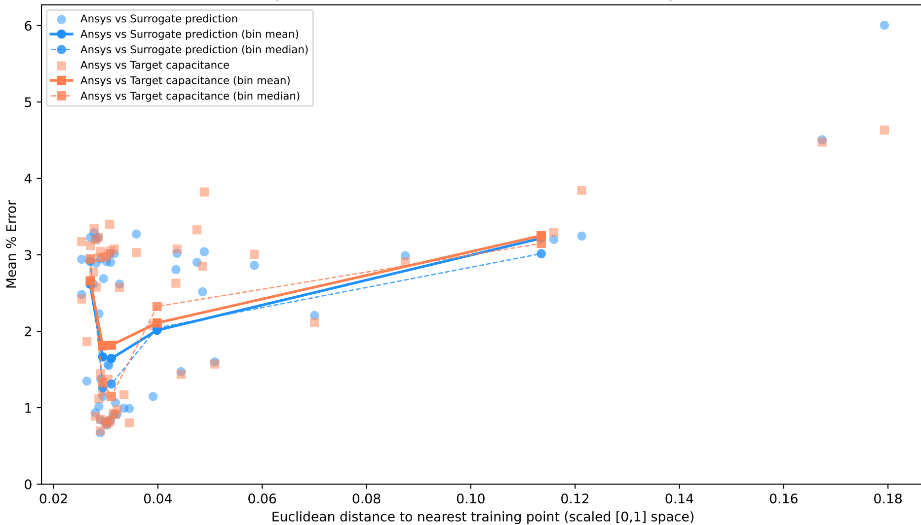
Ansys Validation: Error vs Distance to Nearest Training Point
