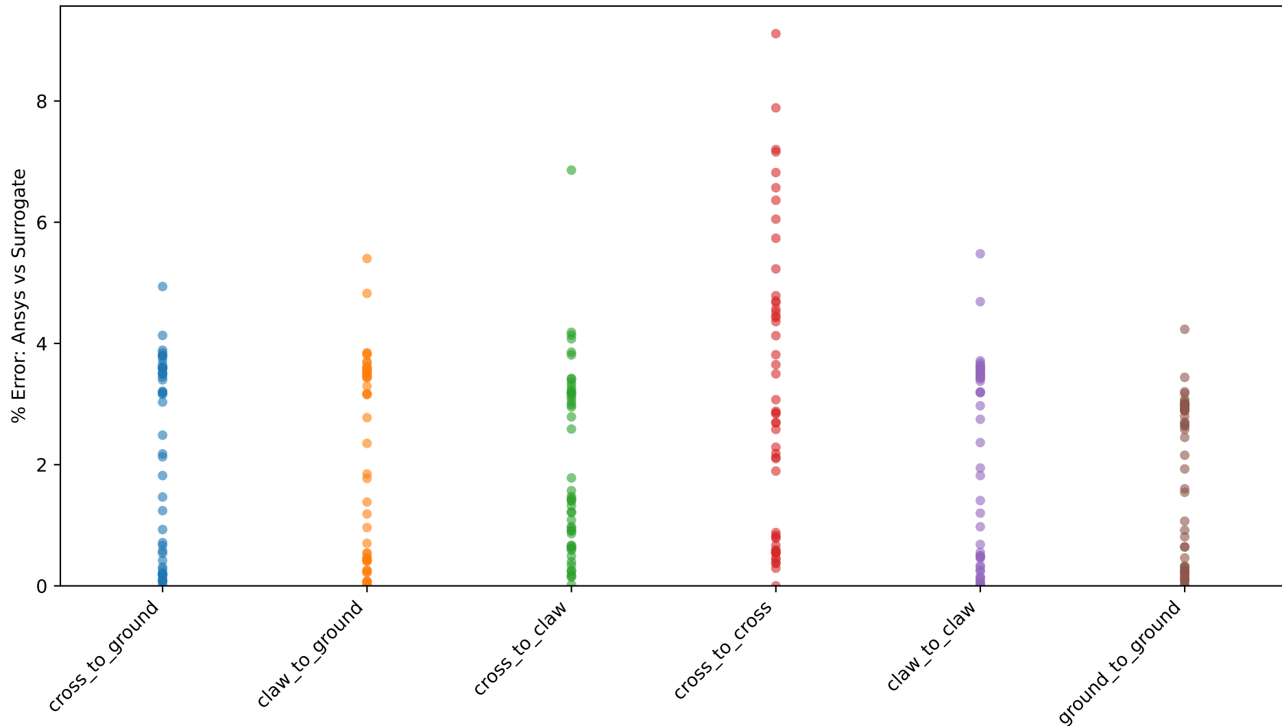
Per-Capacitance Error: Ansys vs Surrogate Prediction (all sigmas)
