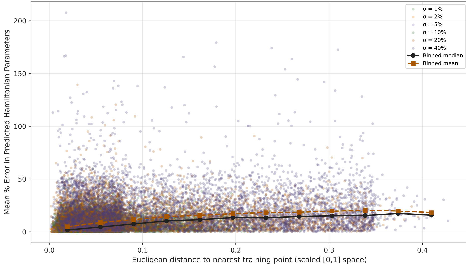
Surrogate Stress Test: Error vs Distance to Nearest Training Point
