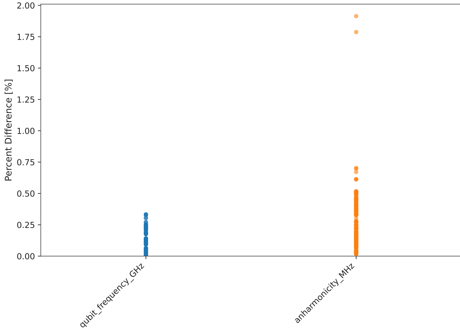
Percent Difference: Hamiltonian
