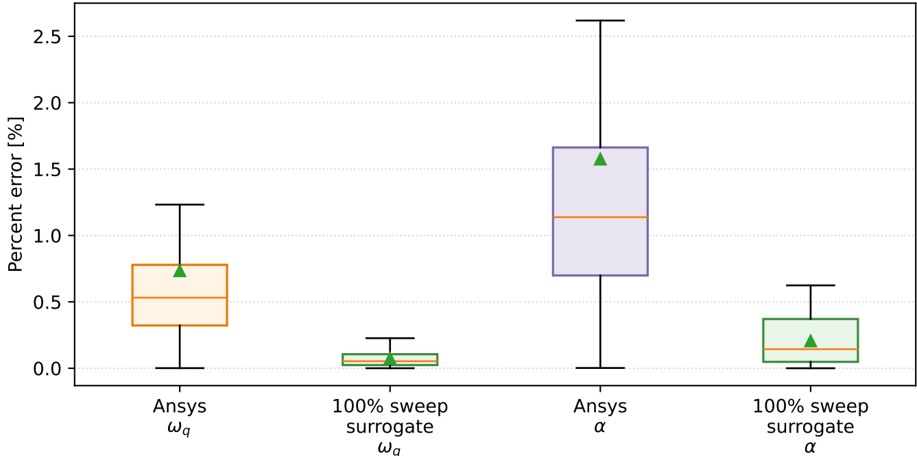
Same Ansys-validation targets: Ansys re-simulation vs 100% sweep model surrogate reconstruction
