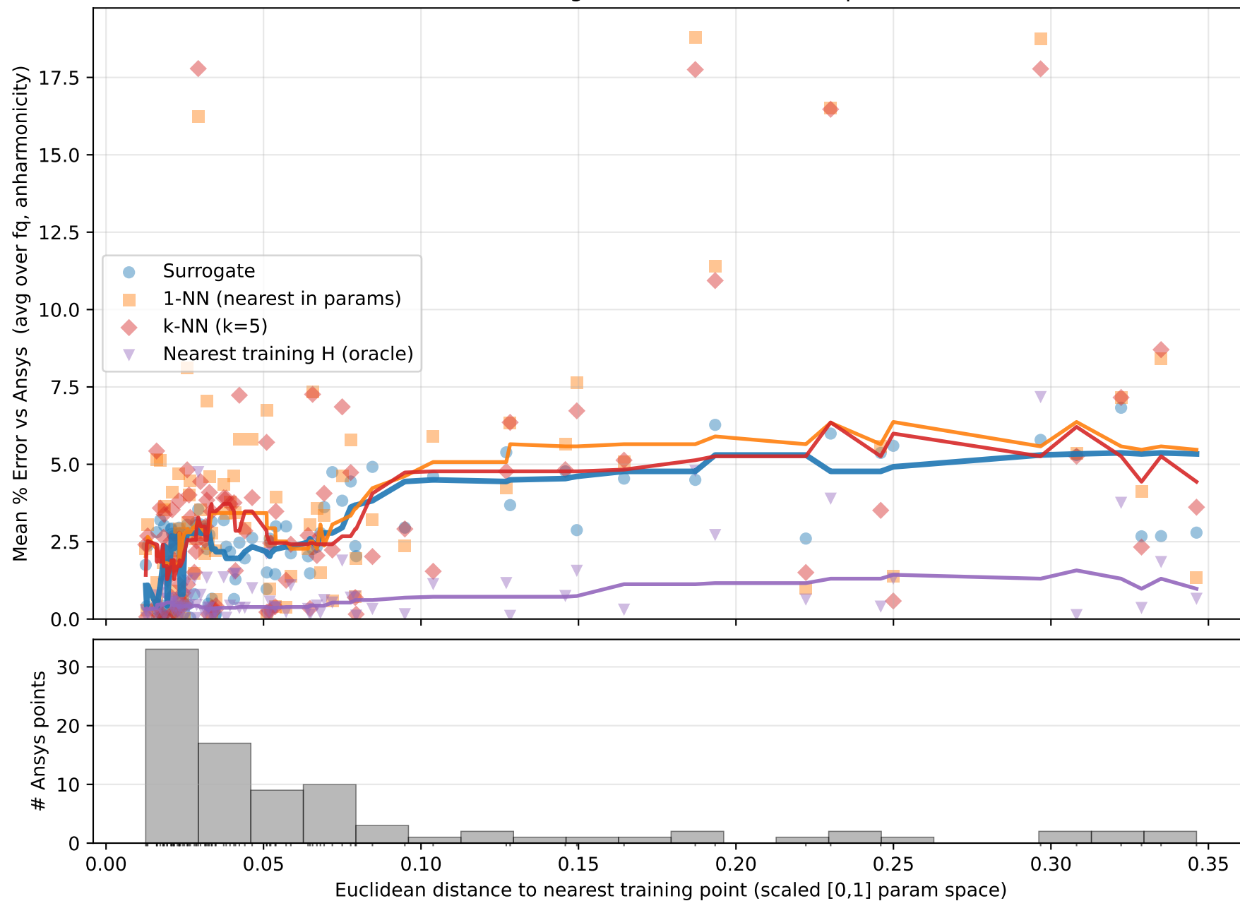
Surrogate vs Classical Interpolation, scored against Ansys HFSS (lines = rolling median, window = 15 points)
