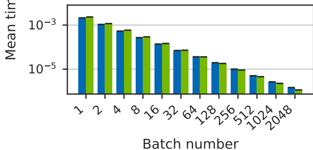
Surrogate only
