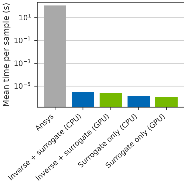
Ansys vs surrogate inference
