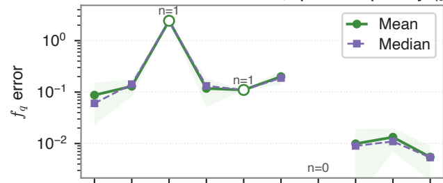
EM simulator validation, qubit frequency ( f_q )
