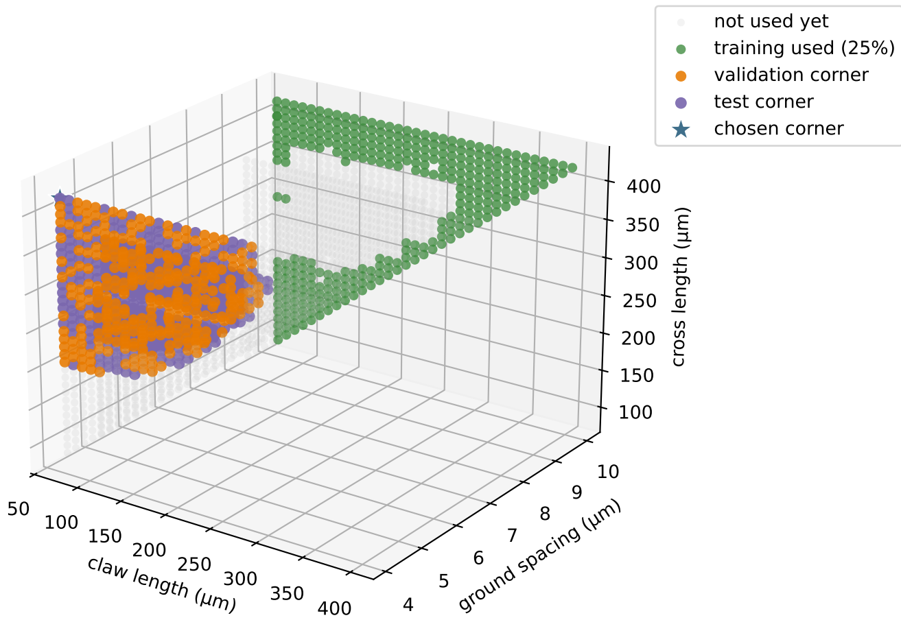
Geometry coverage at 25% training fraction
