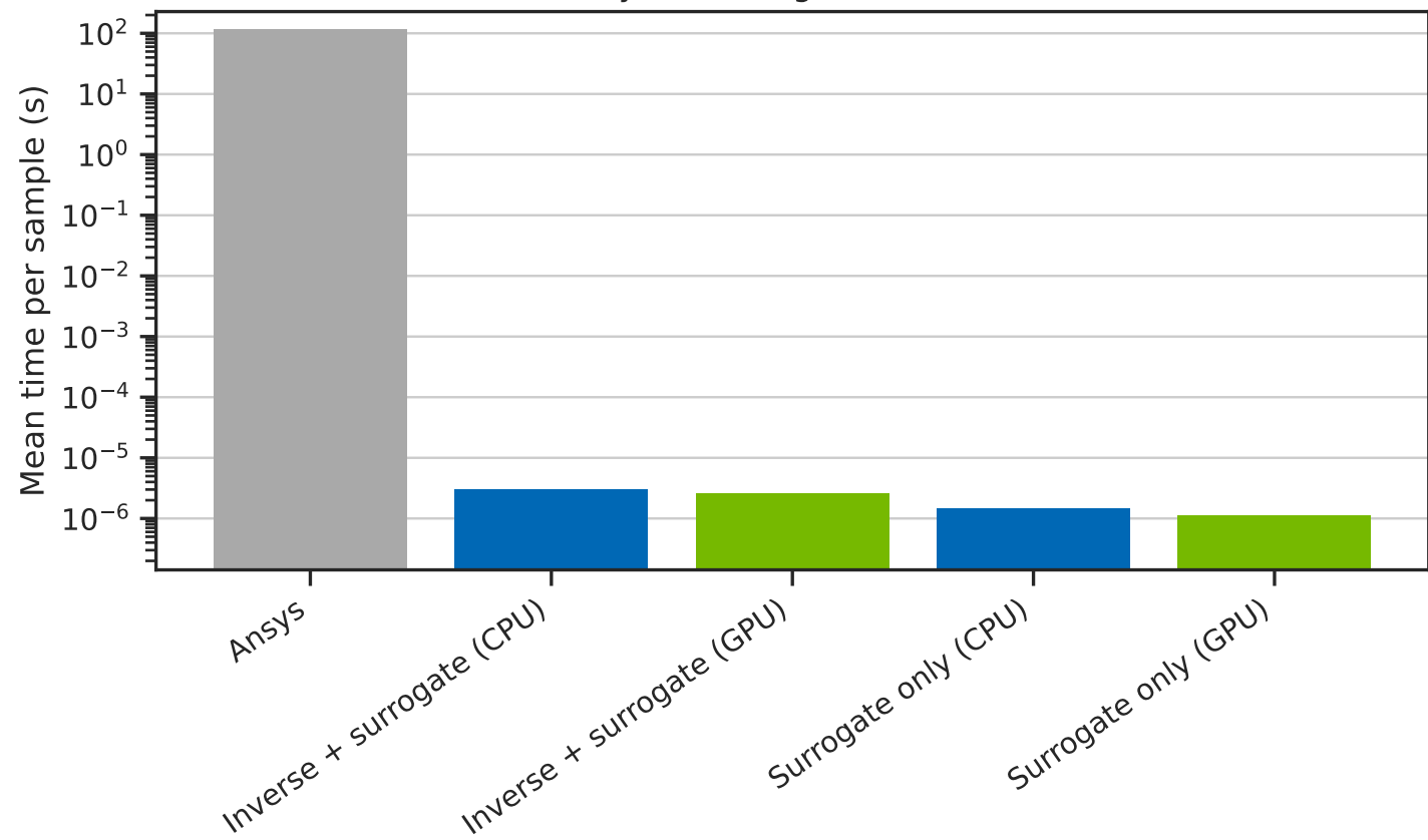
Ansys vs surrogate inference
