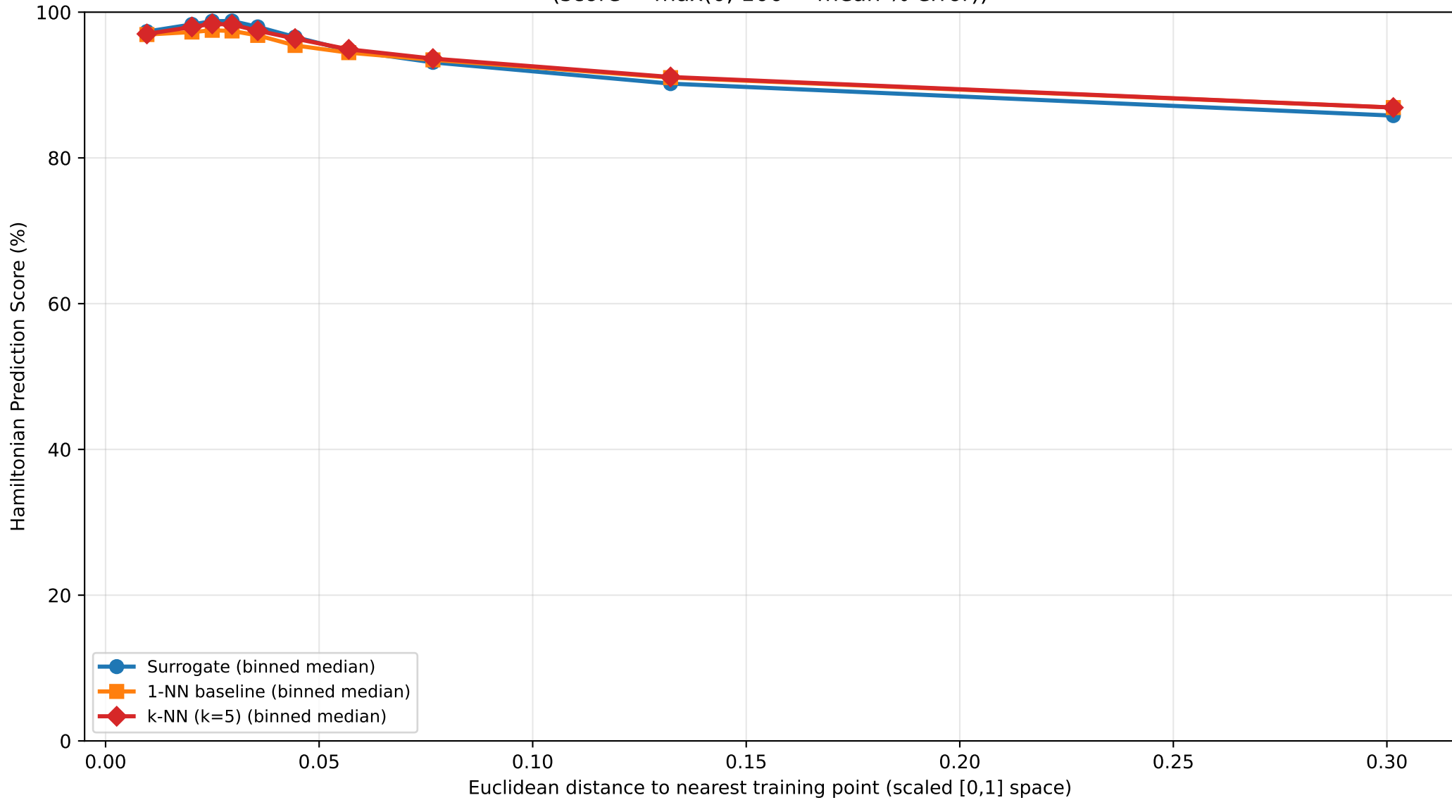
Surrogate vs Classical Interpolation Baselines (score = \max(0, 100 - \text{mean \% error}) )
