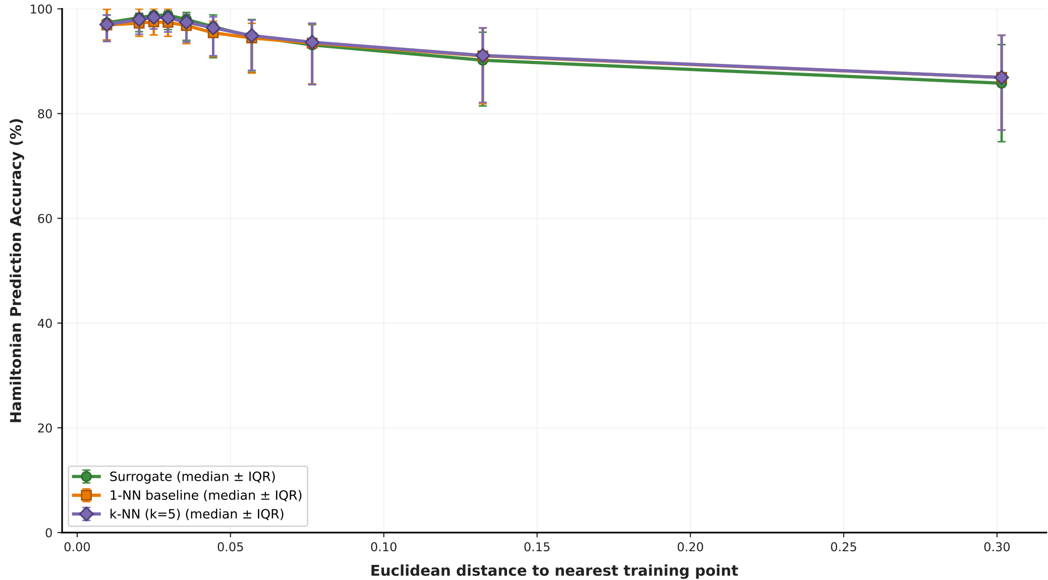
Surrogate vs Classical Interpolation
