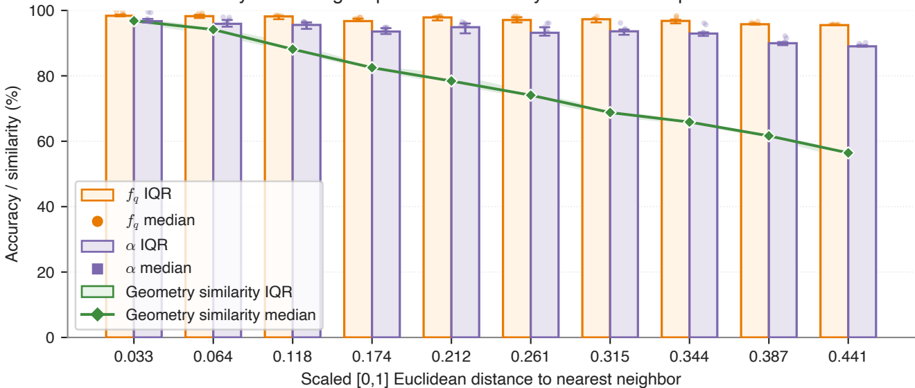
Anslys vs surrogate prediction accuracy of Hamiltonian parameters
